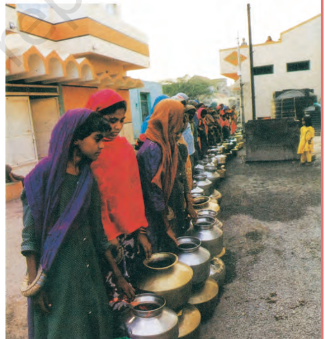
Fig. 3.1: Water Scarcity
